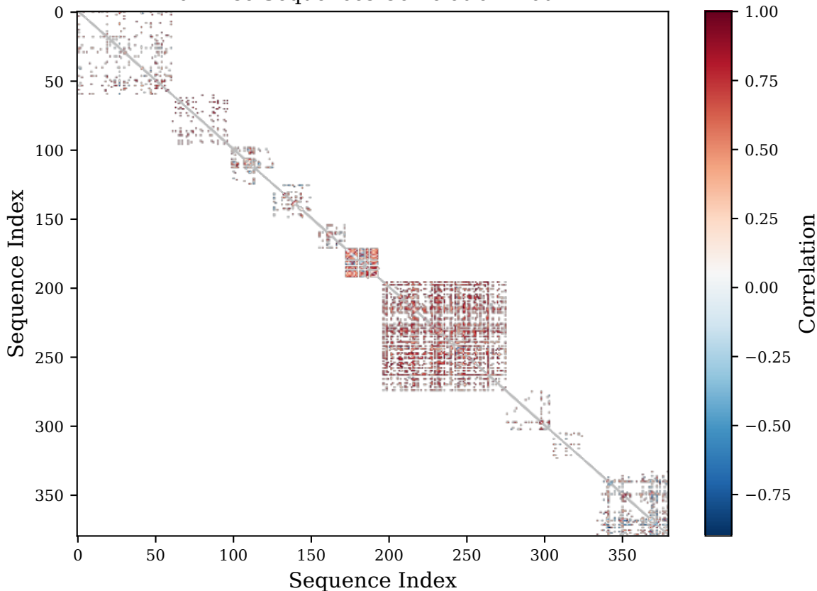
Pairwise Sequences Correlation Matrix
